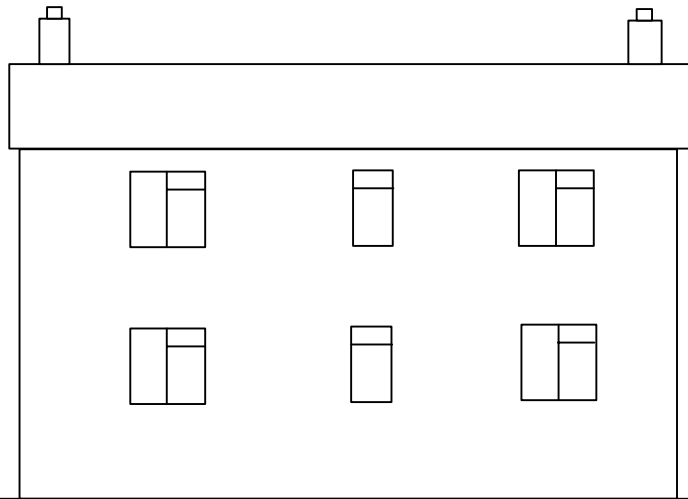
North Elevation - Existing
